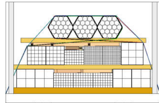
Mixed CHS hex. packs and RHS
