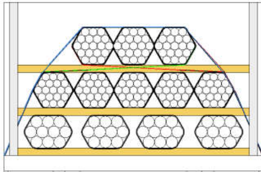
CHS hexagonal packs
